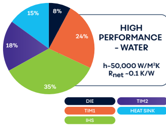
Intel i9 7980E with good TIM1 (0.1 cm 2 K/W) & "so-so" TIM2 (0.25 cm 2 K/W) thermal grease
